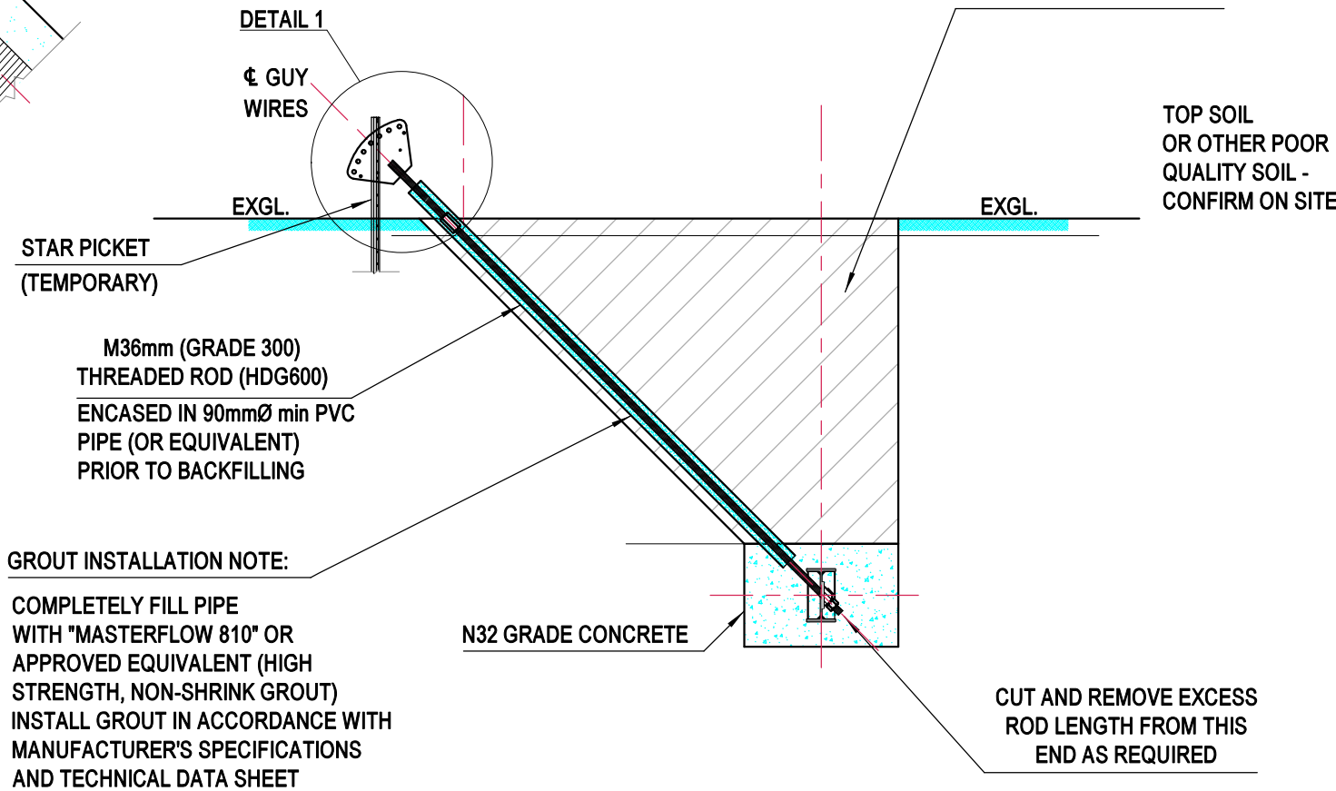
GUY FOOTING SCALE 1:40
